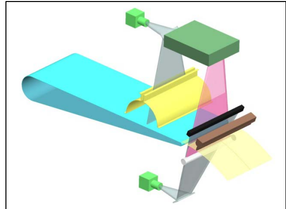
Top Camera, Bottom Camera and Top Laser Sorter Configuration
