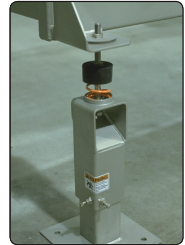
Corner Column
